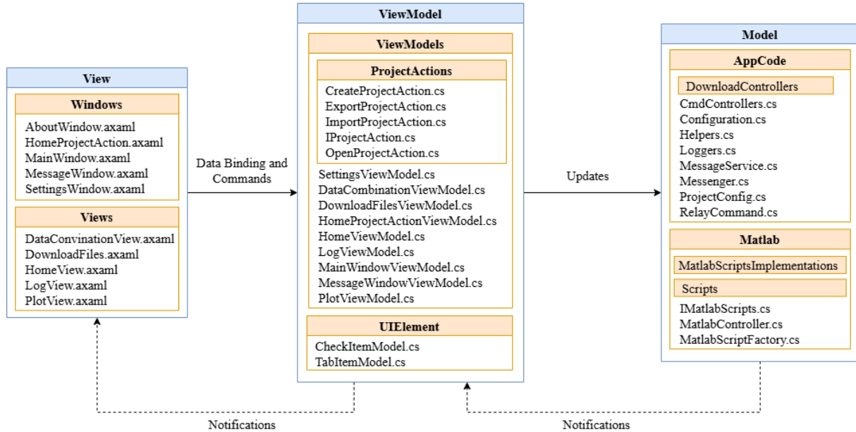
Figure 18: MVVM design pattern applied to the project architecture
