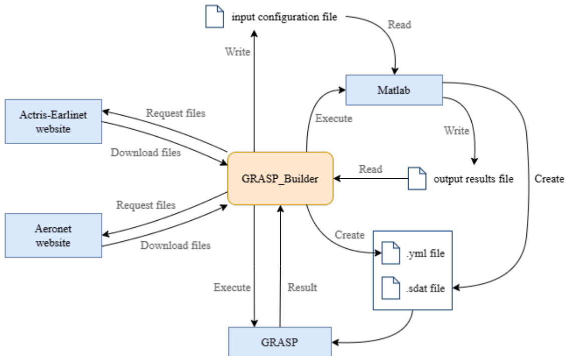
Figure 20: Application interactions diagram
